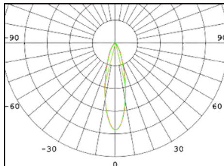
Symmetrical 30° F14503
