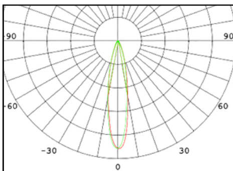
Symmetrical 18° F14502
