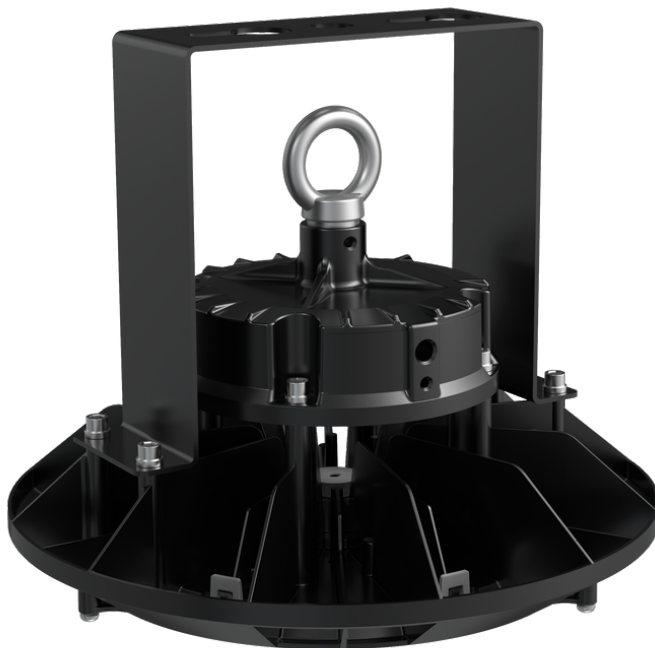
Ceiling Mounting
